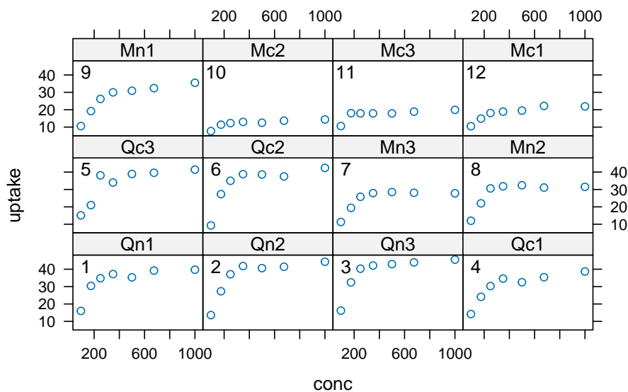
Figure 1: fn$xyplot
